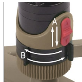
3. a) Adjust up for full circle or down for part circle. b) Adjust left or right to set part-circle arc.
